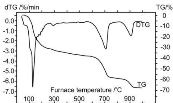
FIGURE 2. Thermogravimetric (TG) and differential thermogravimetric (DTG) curves of slavikite. LabSys TG-DTA/DSC, sample weight 45 mg, 10 °C/min, dynamic He atmosphere, 15 mL/min.
