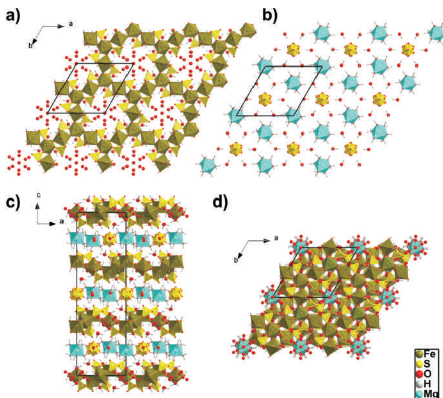
FIGURE 6. Honeycomb-like structure of the Fe-hydroxy-sulfate layer (a), Mg-aqua cations, disordered SO 4 2- anions, and water moieties forming layer (b), the unit cell of slavikite view along the Y axis (c) and Z axis (d).
