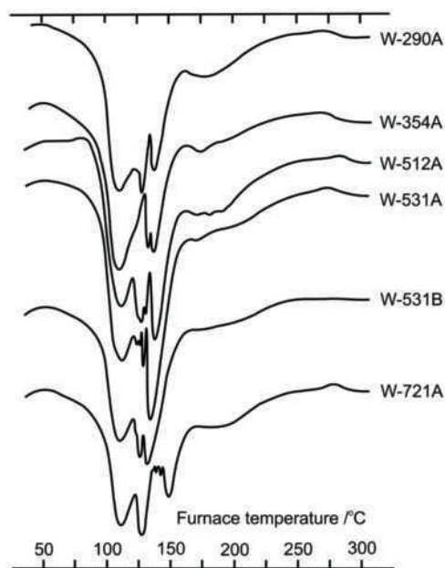
FIGURE 5. Dehydration of selected slavikite samples shown by DTA curves. LabSys TG-DTA/DSC, samples weight 40 mg, 10 °C/min, dynamic He atmosphere, 15 mL/min.
