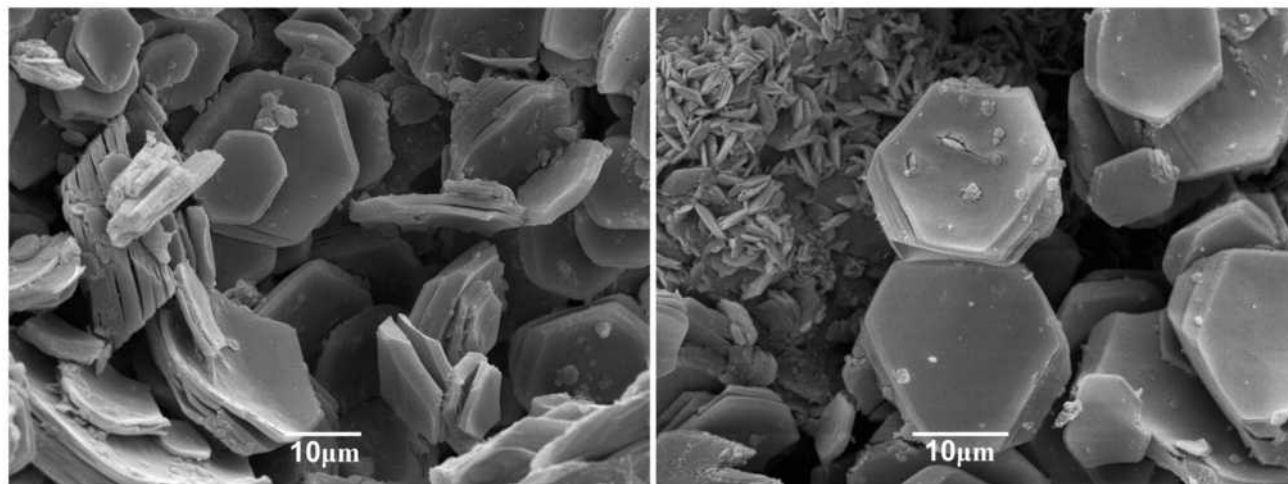
FIGURE 1. SEM images of slavikite crystals from Wieściszowice.
