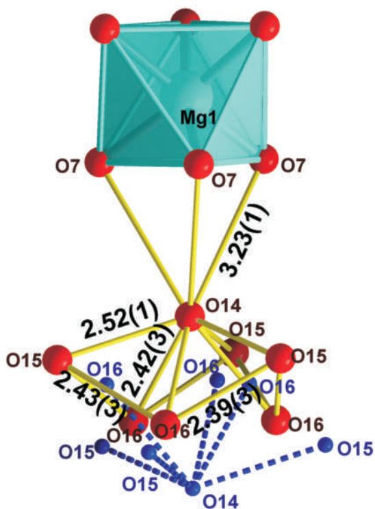
FIGURE 4. A possible assignment of the O···O contacts in the disordered protonated water cluster. The yellow and dashed blue lines represent possible hydrogen bonds in the cluster. The superposition of the yellow and blue states gives the disordered moiety.
