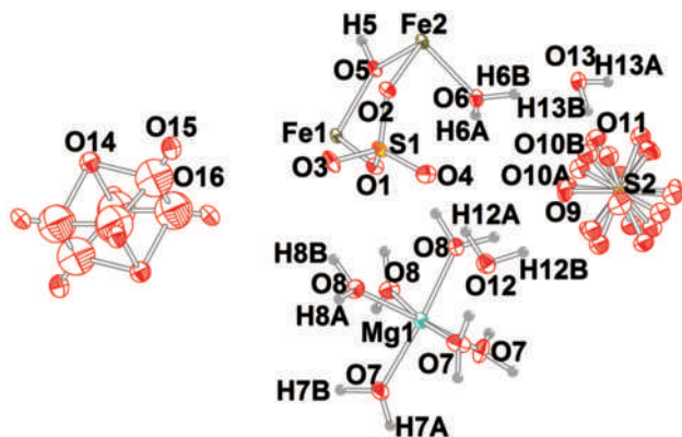
FIGURE 7. Thermal ellipsoids at the 50% probability level.
